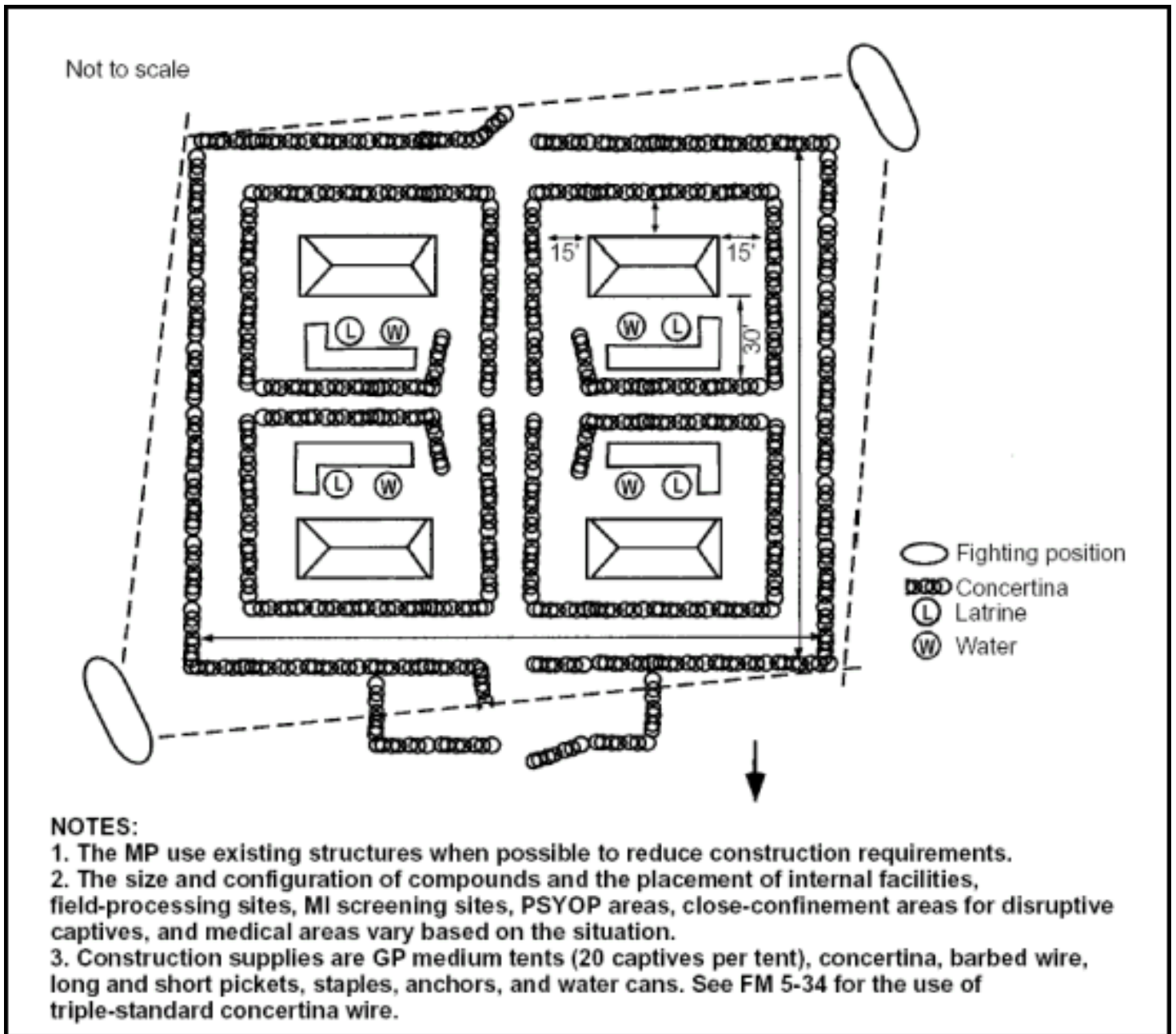
Figure 3-3. Central CP
