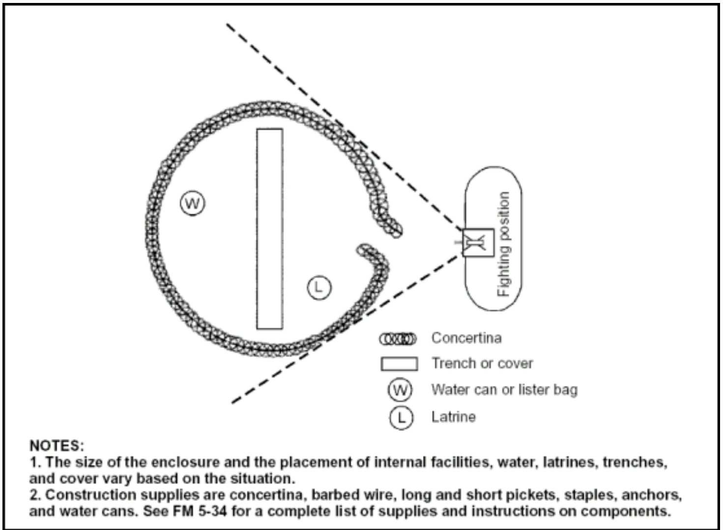
Figure 3-2. Forward CP
